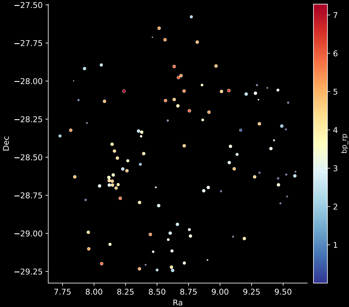
APOGEE DR17 Field: [001-01] Stars: 106
