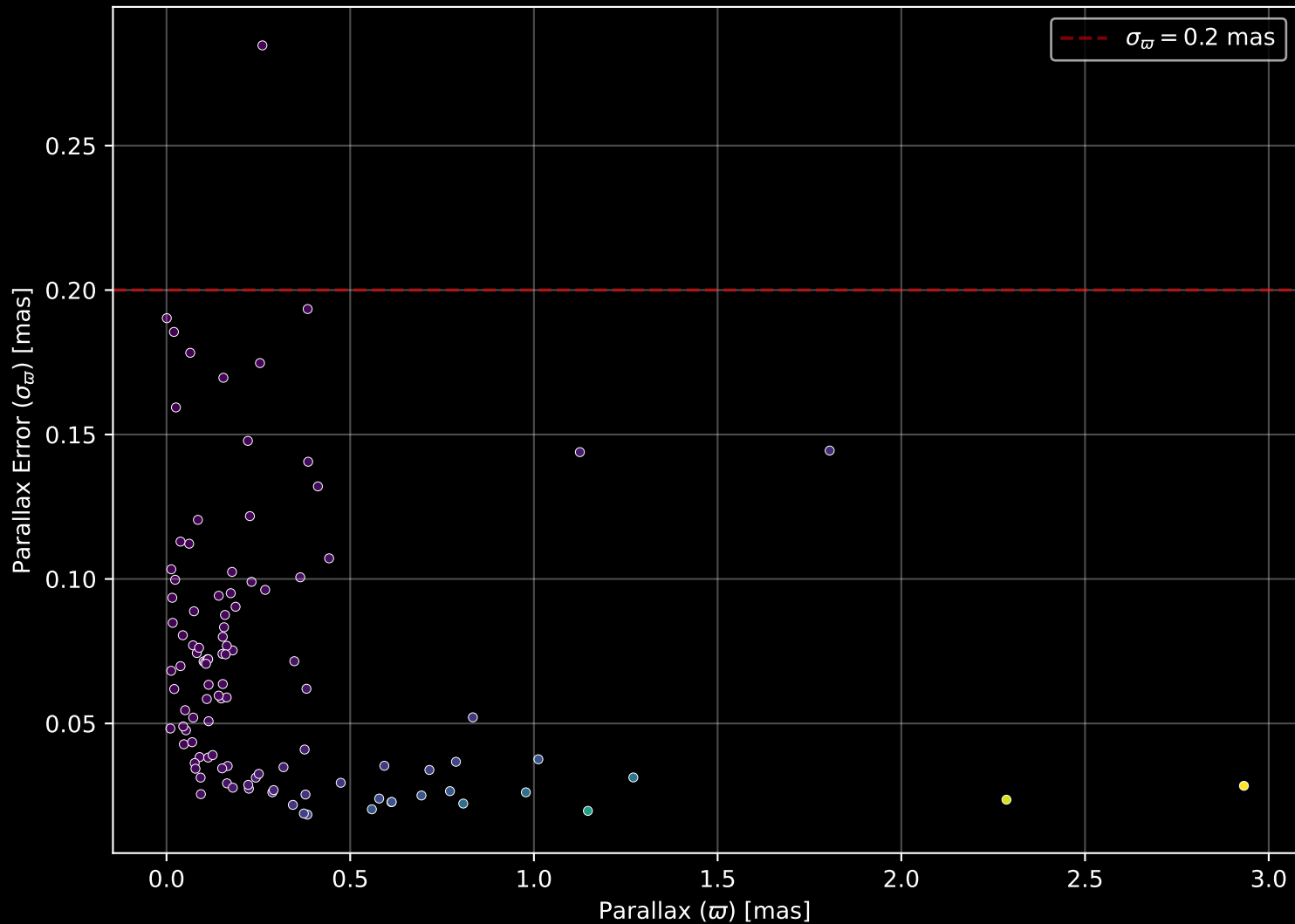
APOGEE DR17 Field: [001-01] Parallax Quality (n= 106)
