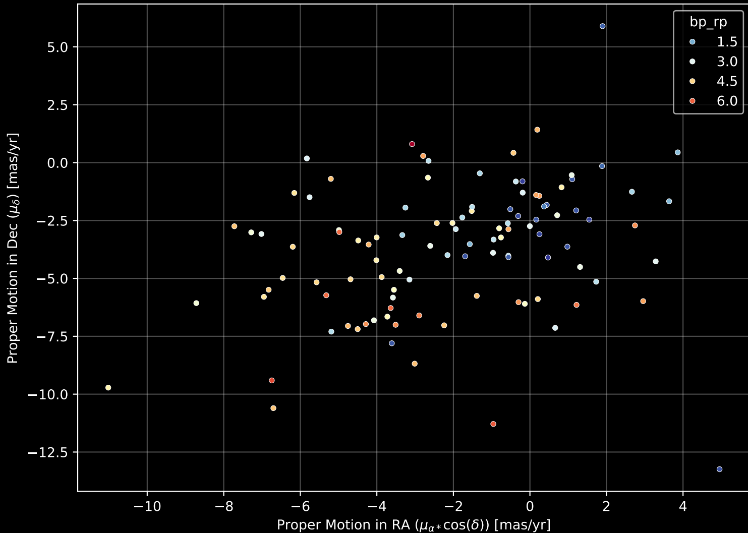
APOGEE DR17 Field: [001-01] Proper Motion Diagram (n= 106)
