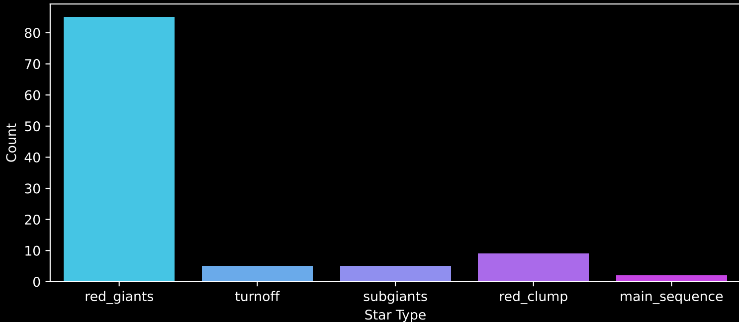
APOGEE DR17 Field: [001-01] Count plot of Star Type
