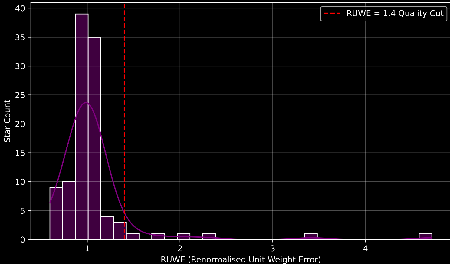
GAPOGEE DR17 Field [001-01] RUWE Distribution (n= 106)
