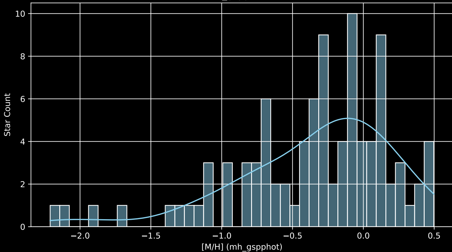
APOGEE DR17 Field: [001-01 [M/H] (mh_gspphot) (n= 95)
